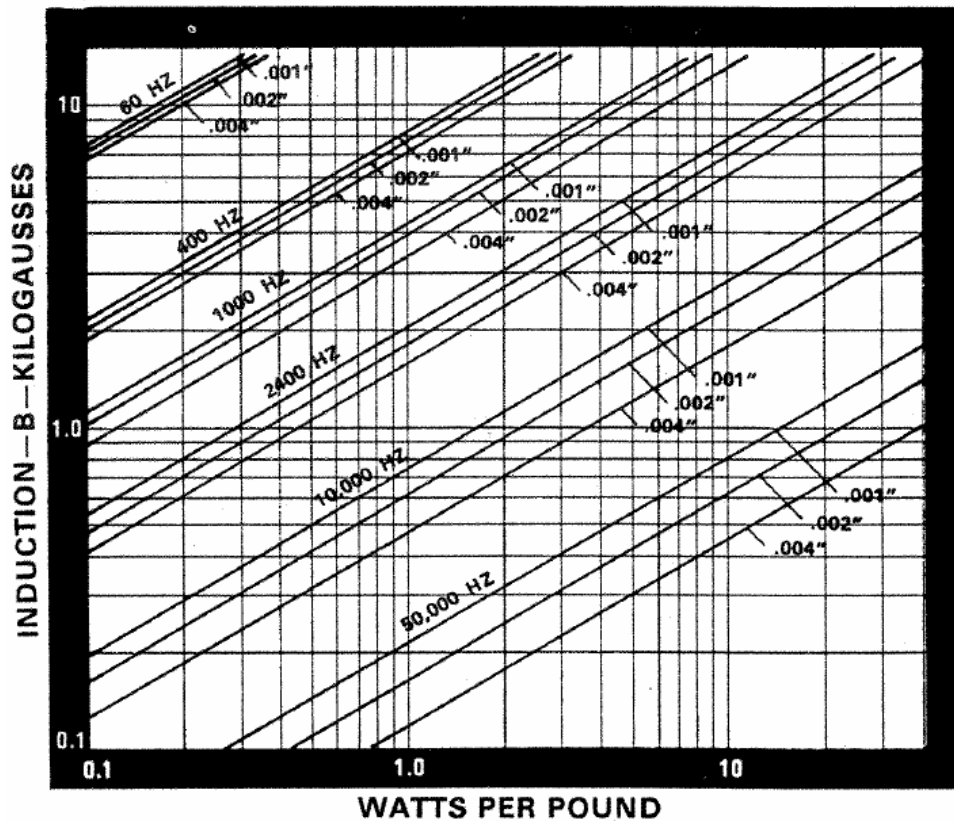
Fig. 23. Core losses for Deltamax
