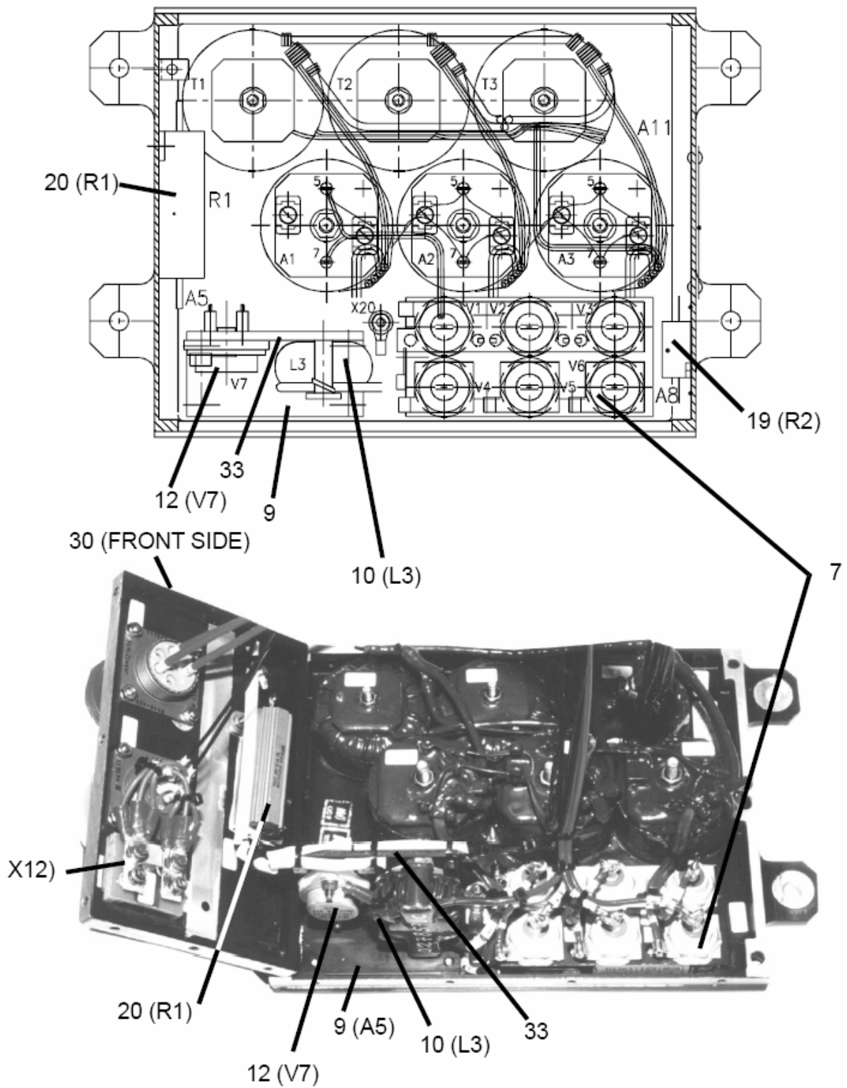
Fig. 27. The layout for three-phase magamp (photo Euroatlas)
