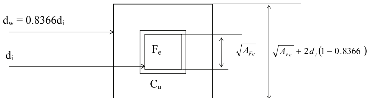
Fig. 46. The copper winding, cross section.
