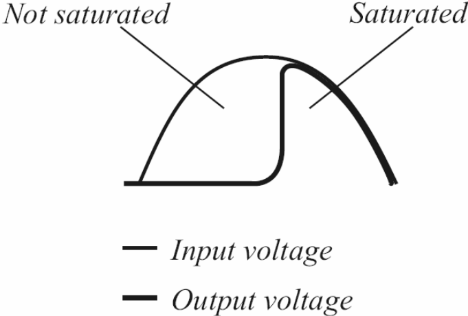
Fig. 13. Example of a wave form occurring in a magnetic switch during operation
