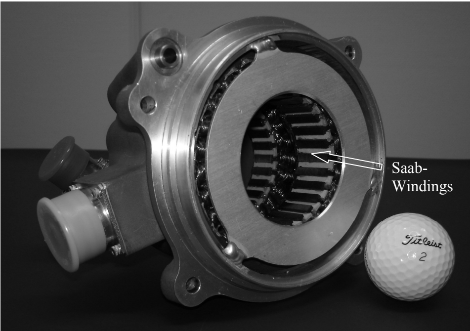
Fig. 53. The stator for the PM-generator used in JAS39 Gripen
