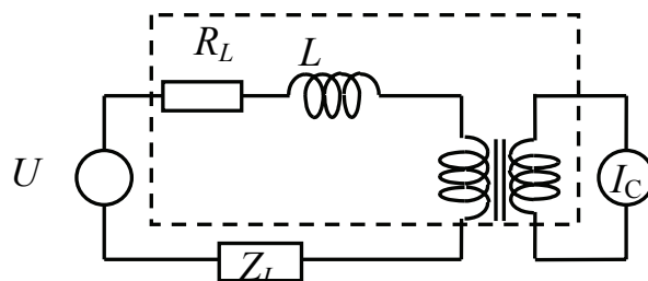
Fig. 31. Equivalent circuit of one phase of a simple magnetic amplifier
