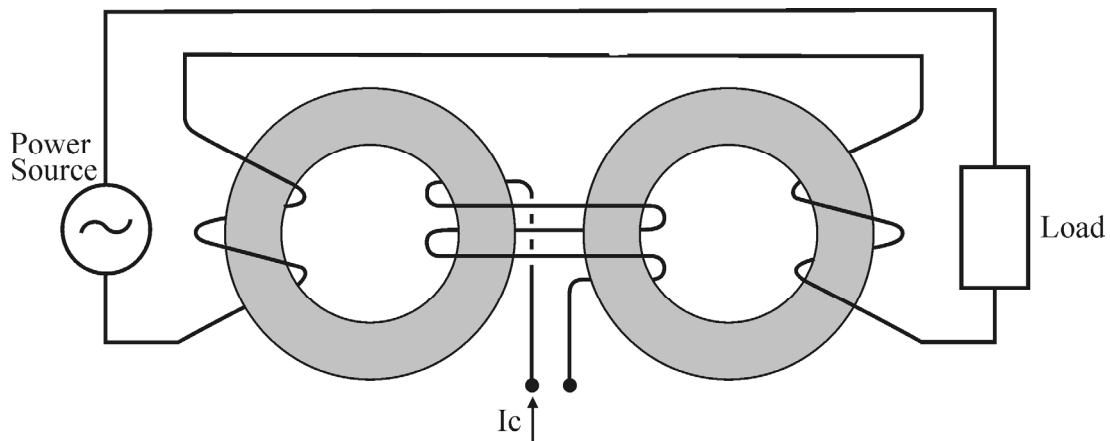
Fig. 7. Two cores with a common control winding
