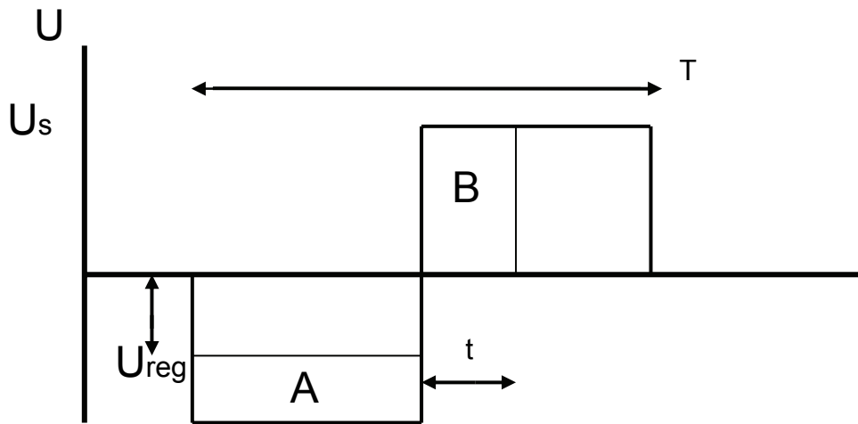
Fig. 15b. The operation characteristics for the Ramey magamp
