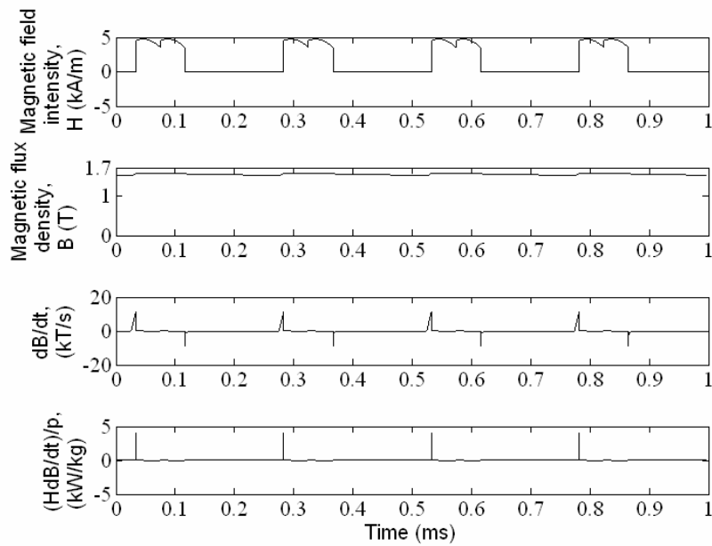
Fig. 38. Simulated field quantities and losses as functions of time for loop A
