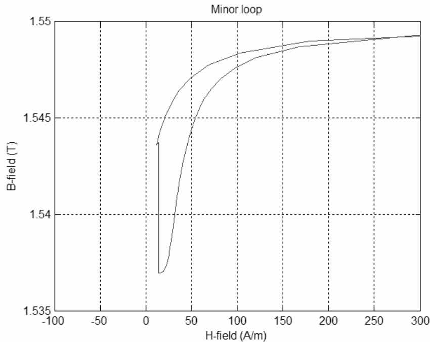
Fig. 43. A detailed simulation with a control current I_C of -100mA
