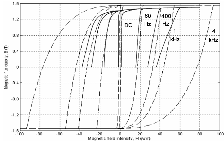
Fig. 36. Hysteresis model for Metglas 2605 TCA/S-2 Characteristics for different frequencies. The solid lines are the producers data, the dashed lines are major loops generated by the model.
