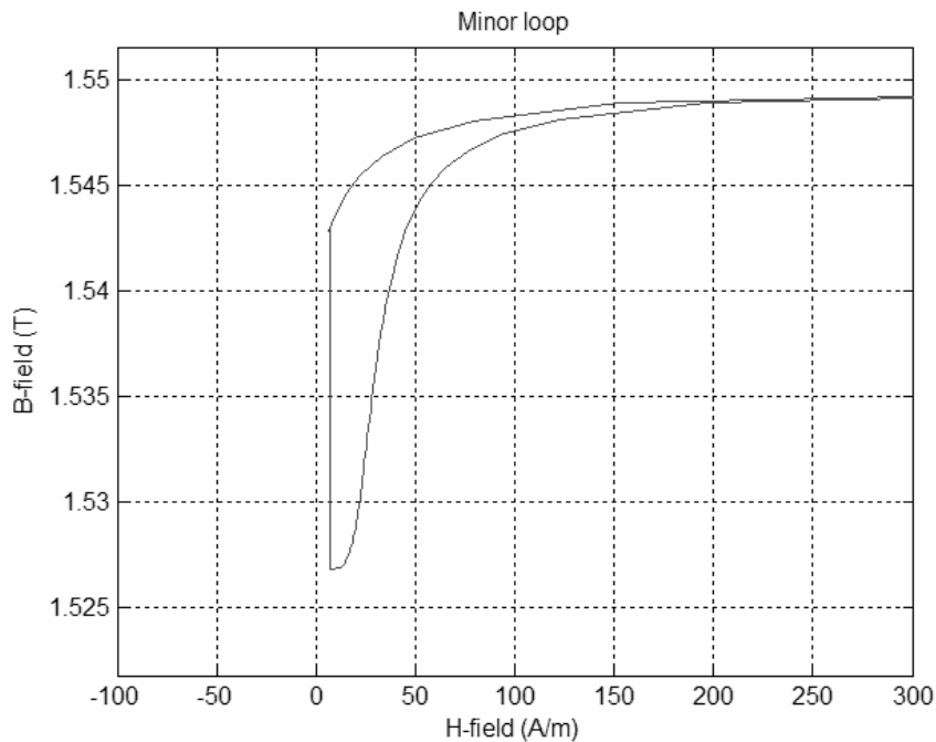
Fig. 42. A detailed simulation with a control current I_C of -50mA
