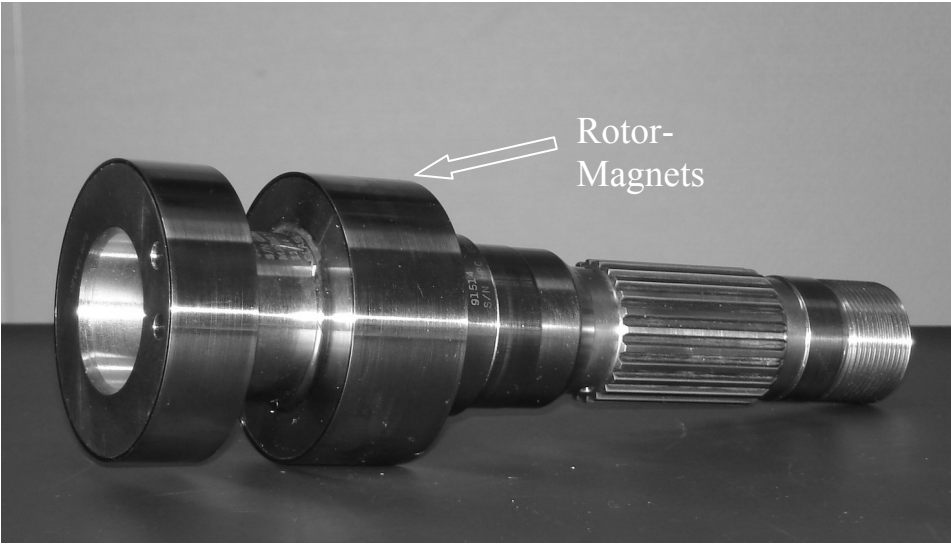
Fig. 54. The rotor for the PM-generator used in JAS39 Gripen
