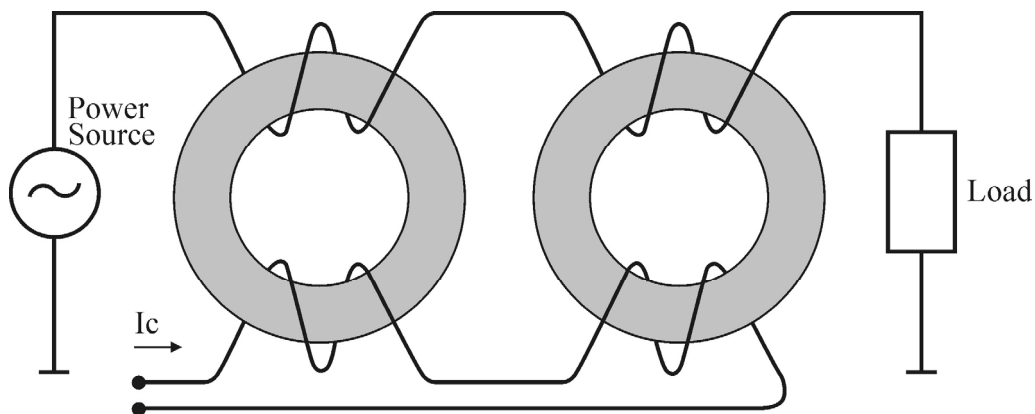
Fig. 6. The two core magnetic switch
