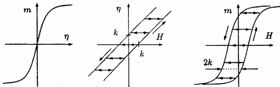
Fig. 32. The anhysteretic curve is shown to the left. In the middle the play operator function is illustrated. To the right the play function is combined with the anhysteretic curve giving the hysteresis model of a single pseudo particle.
