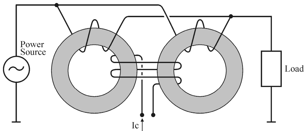
Fig. 8. Two cores with parallel power windings
