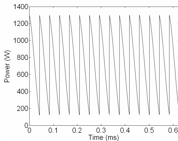
Fig. 44. Output power characteristics corresponding to loop B
