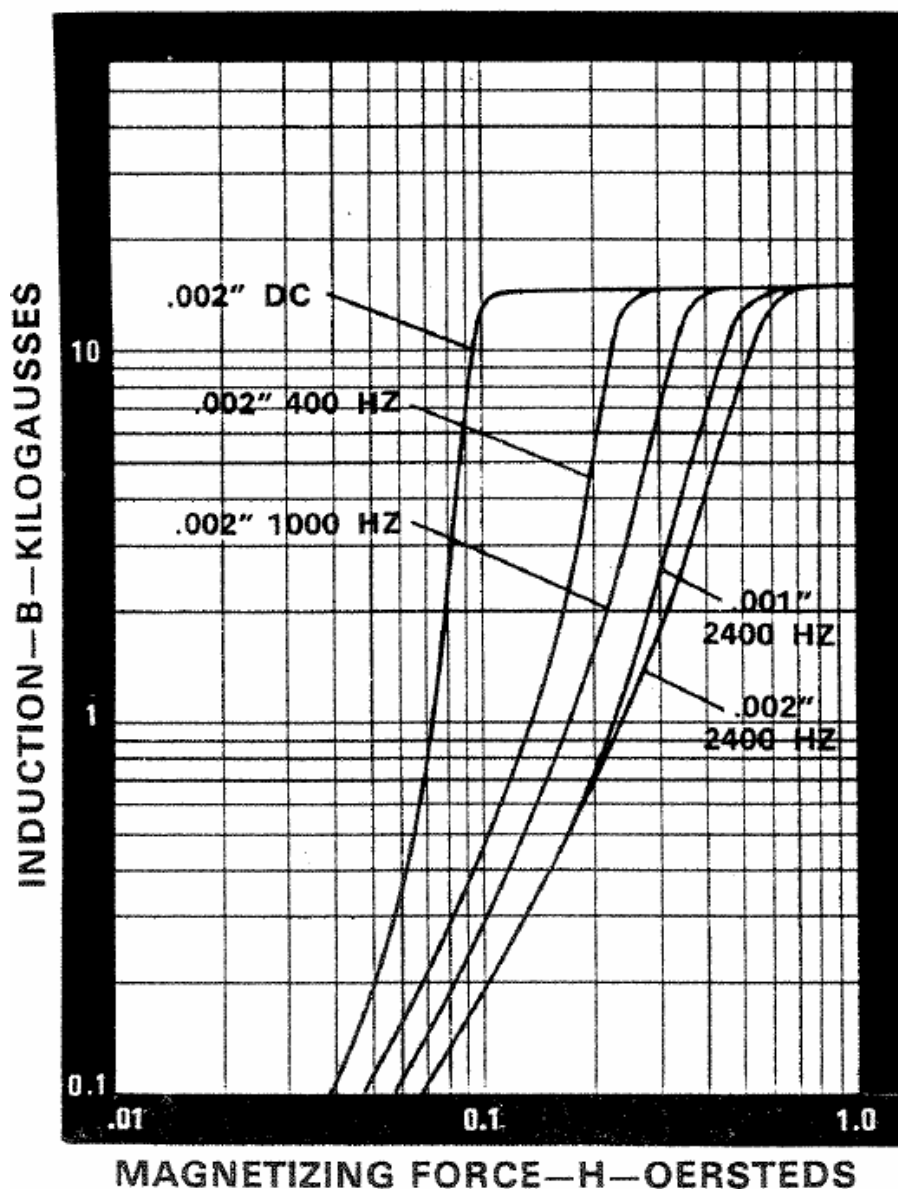
Fig. 21. Deltamax characteristics
