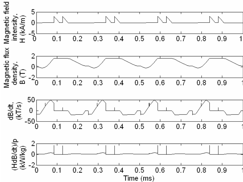
Fig. 40. Simulated field quantities and losses as functions of time for loop C
