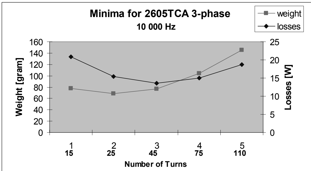
Fig. 50. Case 3 giving split minimum
