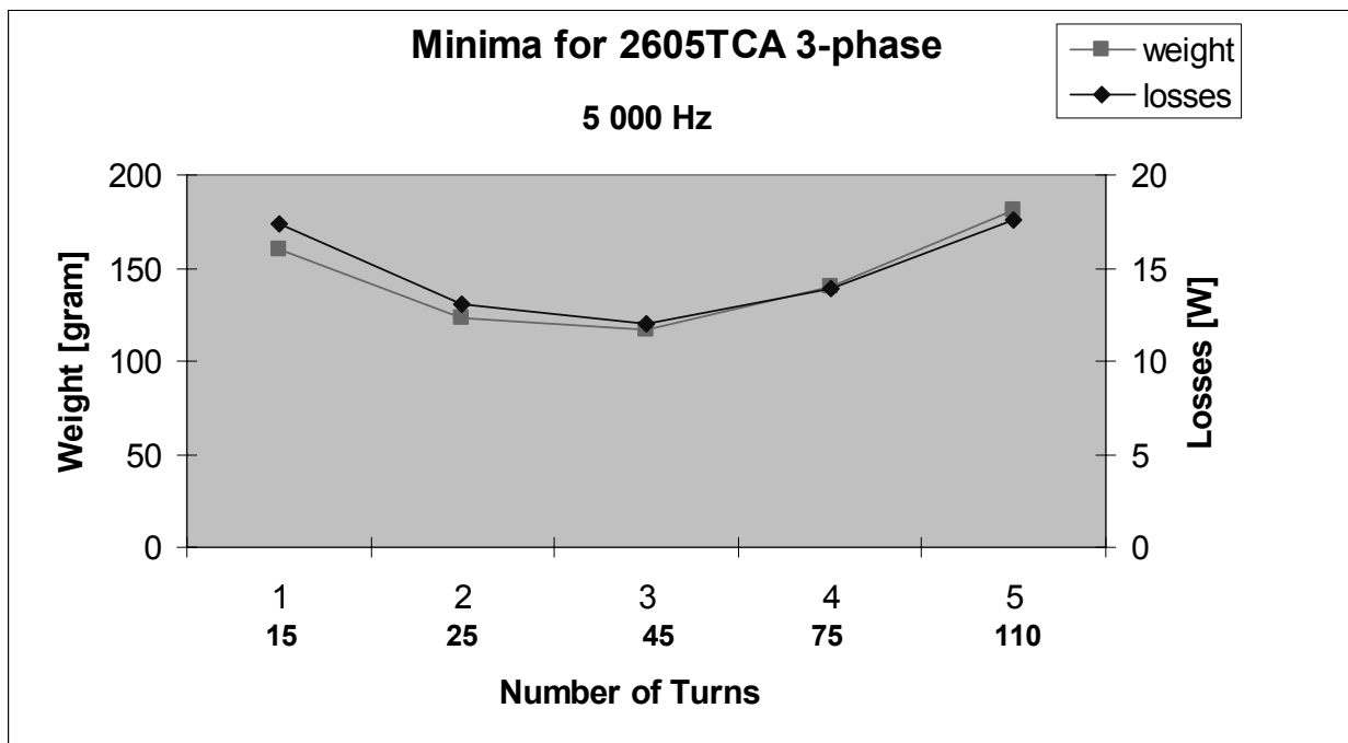
Fig. 49. Case 2 giving coinciding minimum
