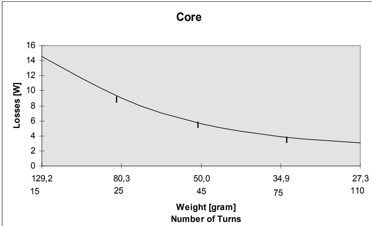
Fig. 45. The core losses for 2605TCA
