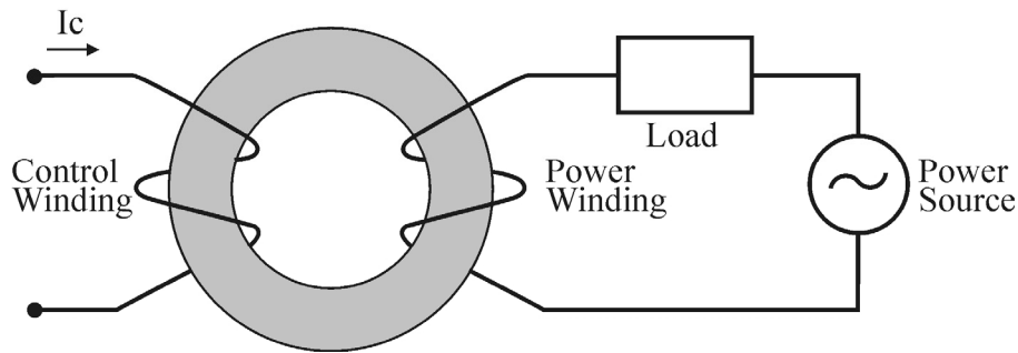
Fig. 5. The one-core magnetic switch
