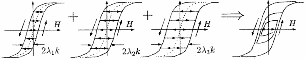
Fig. 33. Weighted superposition of the contribution from minor loops
