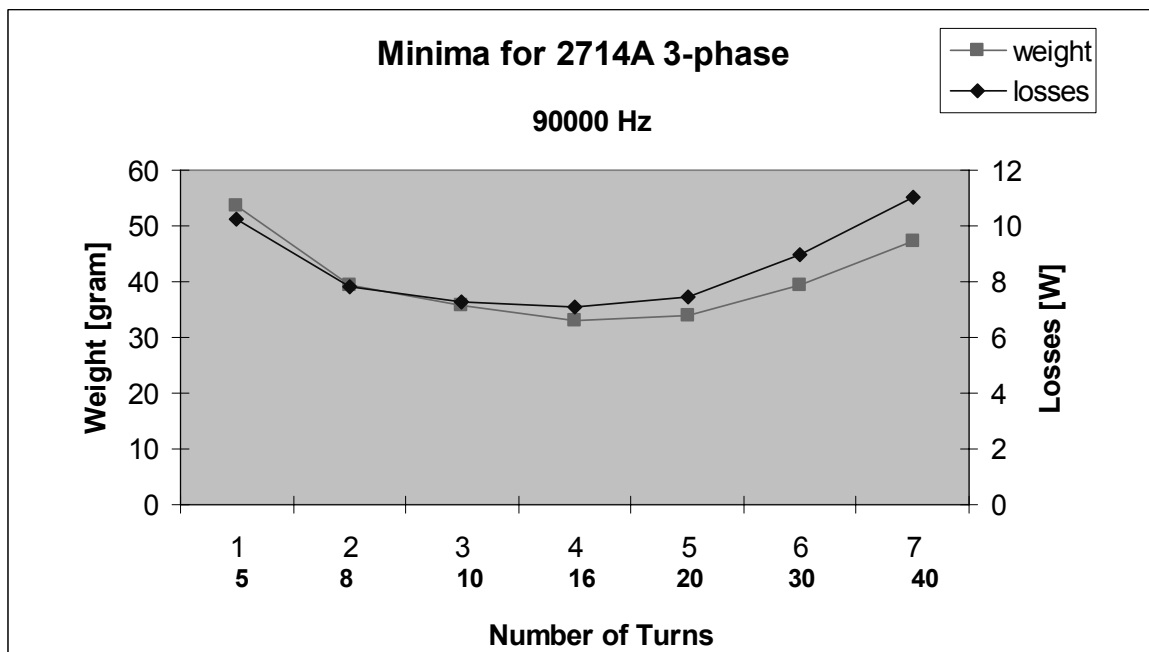
Fig. 52. Case 5 giving coinciding minima
