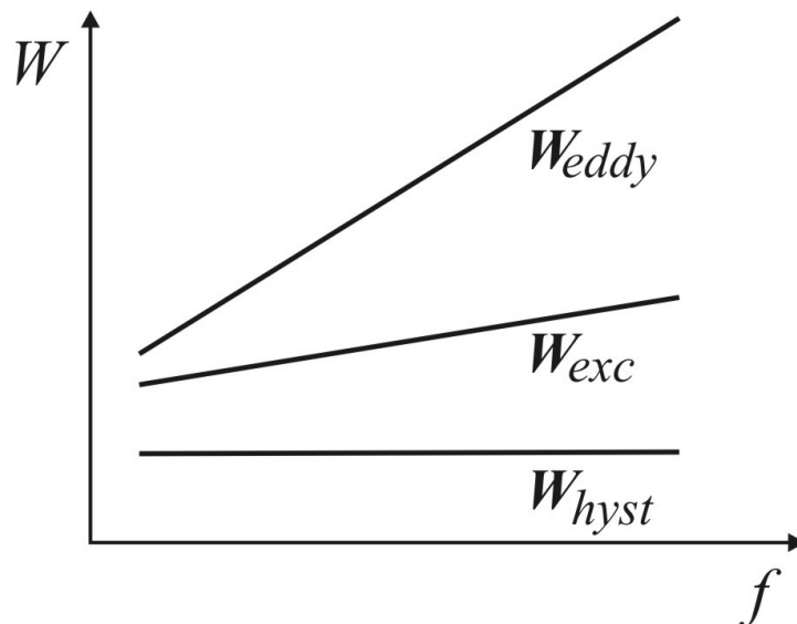
Fig. 24. The energy per cycle separated in different losses
