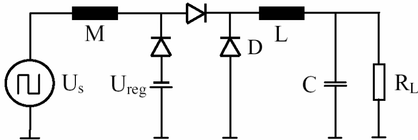
Fig. 14. The one-phase Ramey magamp
