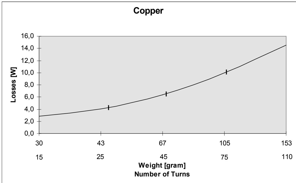
Fig. 47. The copper losses
