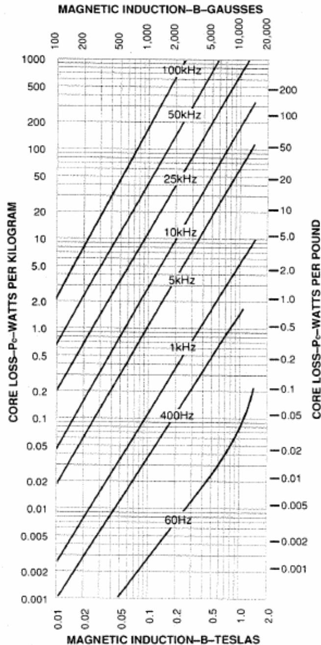
Fig. 22. Core losses for Metglas 2605 TCA
