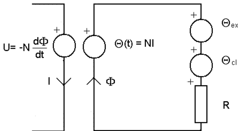
Fig. 34. A winding component circuit model of a single wound core with N turns
