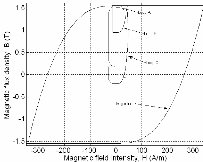
Fig. 37. Minor loop simulation at 4 kHz
