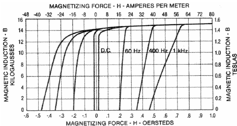
Fig. 20. Metglas 2605TCA characteristics
