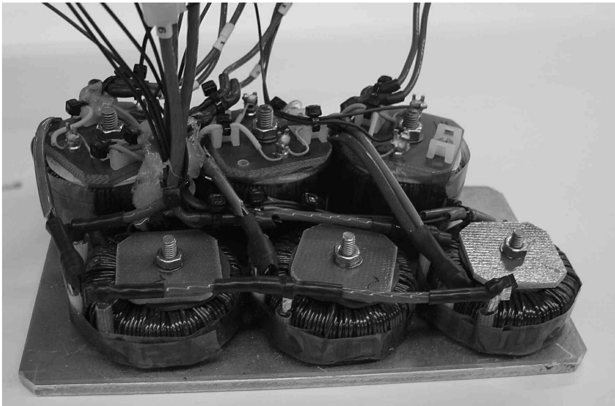
Fig. 26. The wound components in the three-phase magamp (photo Euroatlas)
