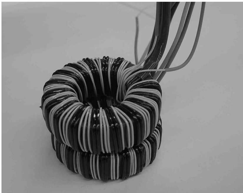
Fig. 10. A two core magnetic switch with separate control windings ( Euroatlas)
