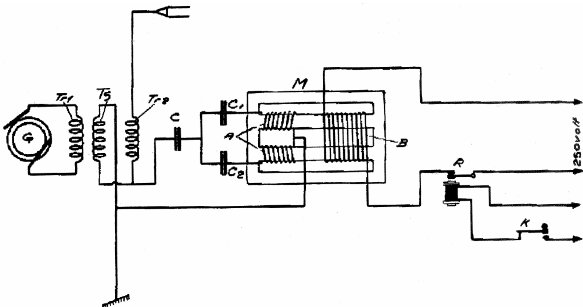
Fig. 4. Circuit diagram for Magnetic amplifier in Grimeton transmitter
