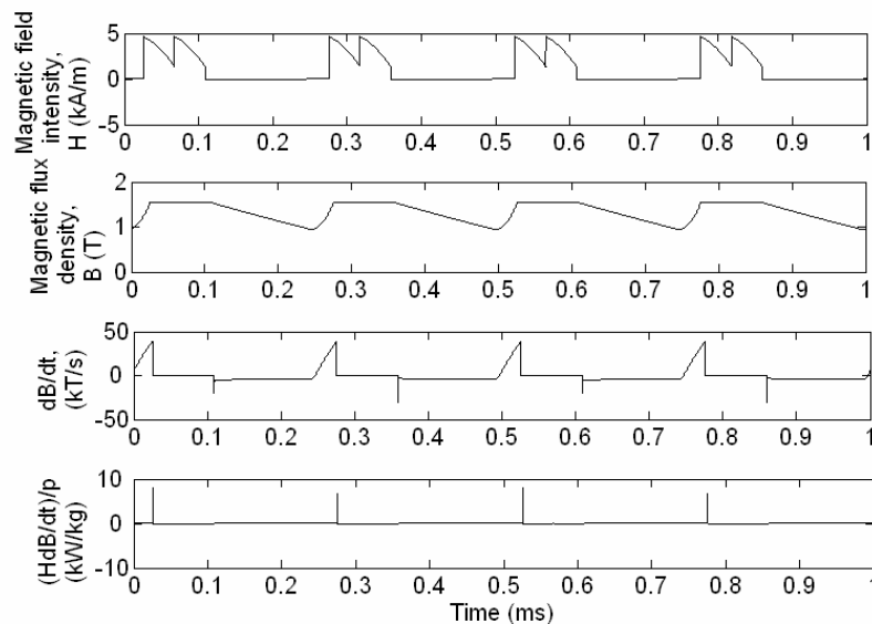
Fig. 39. Simulated field quantities and losses as functions of time for loop B
