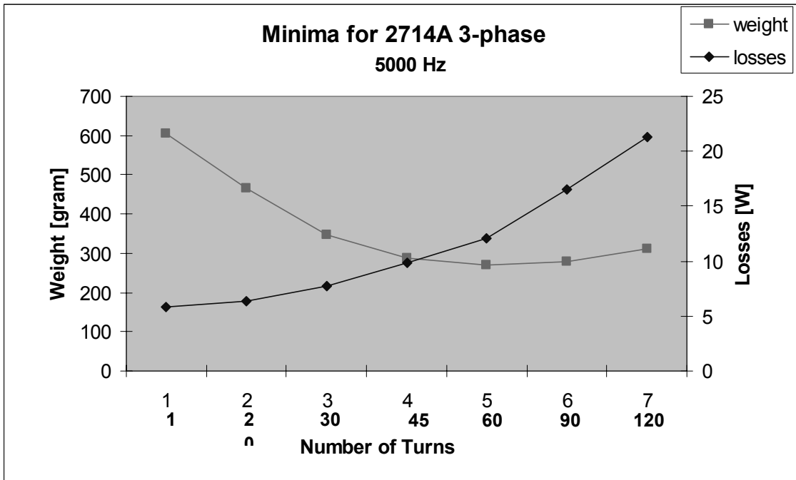
Fig. 51. Case 4 giving of split minima
