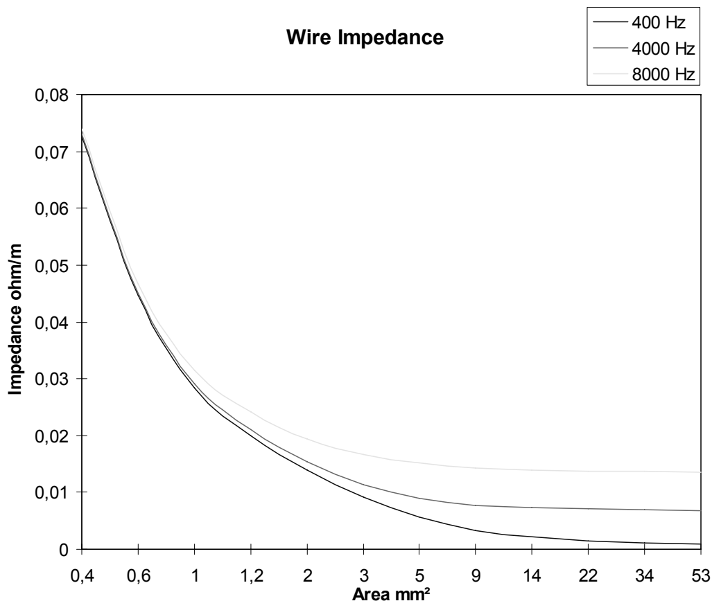
Fig. 56. Shows the absolute value of the one phase wire impedance, for a three phase system as a function of the conductor copper area for d/a=3
