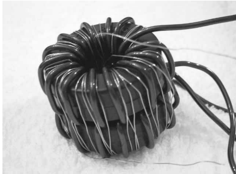
Fig. 11. Example of a two core magnetic switch with one control winding
