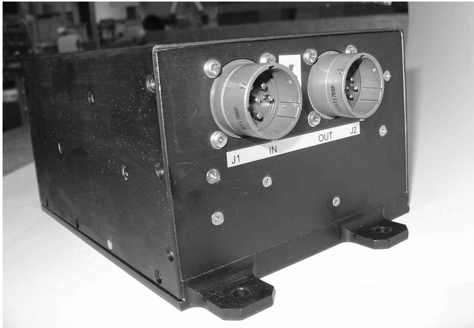
Fig. 29. The magnetic amplifier completed (photo Euroatlas)
