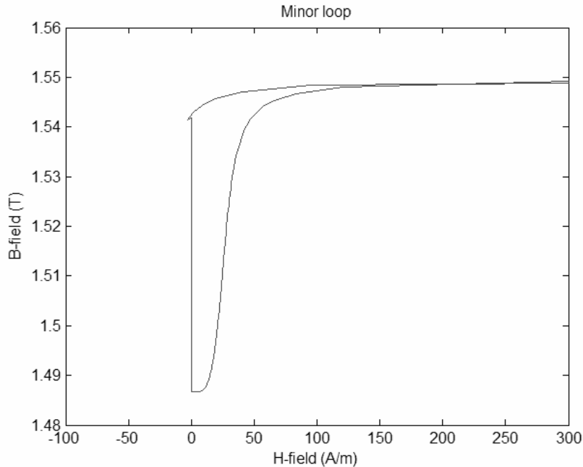
Fig. 41. A detailed simulation with a control current of I_C = 0 mA
