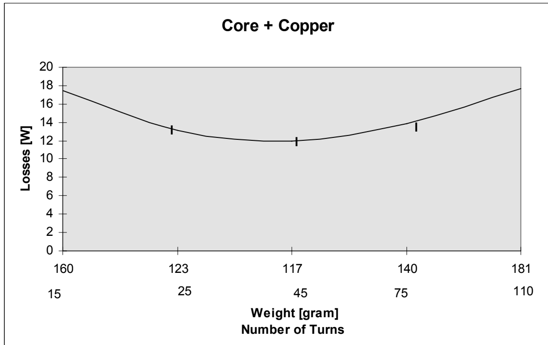
Fig. 48. The core and copper losses
